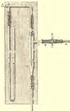
FIG. 6.—Bunsen's Air Suction Pump.
